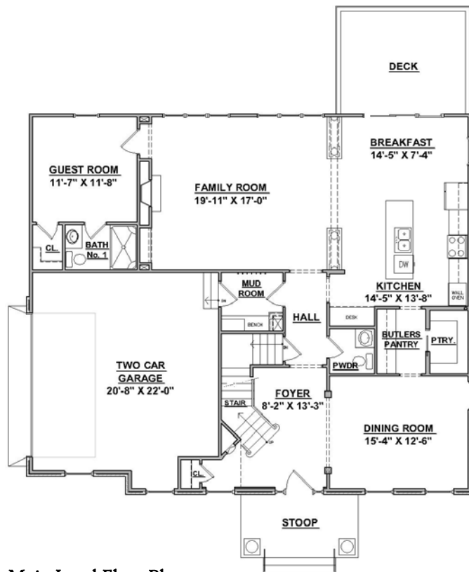
Main Level Floor Plan 1564 square feet
